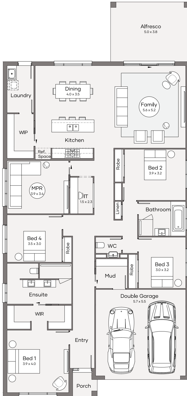
Floor plan
