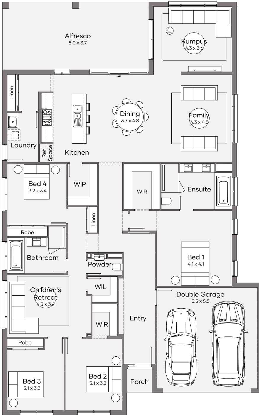
Floor plan
