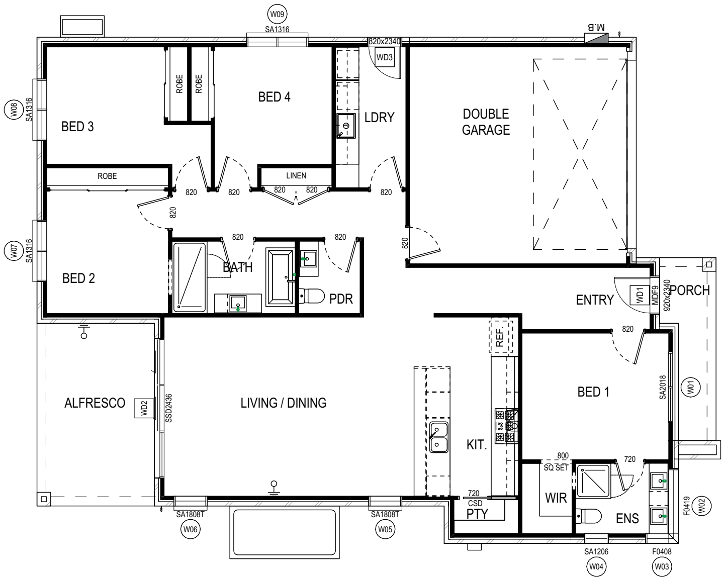
Floor plan
